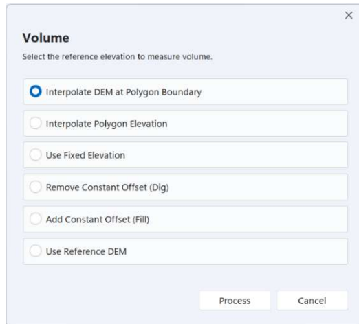
Figure 9: Volume window.
